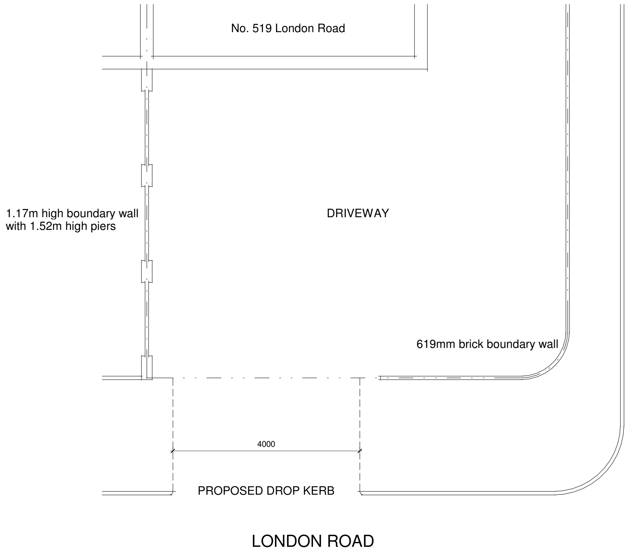
Driveway 1 : 50
