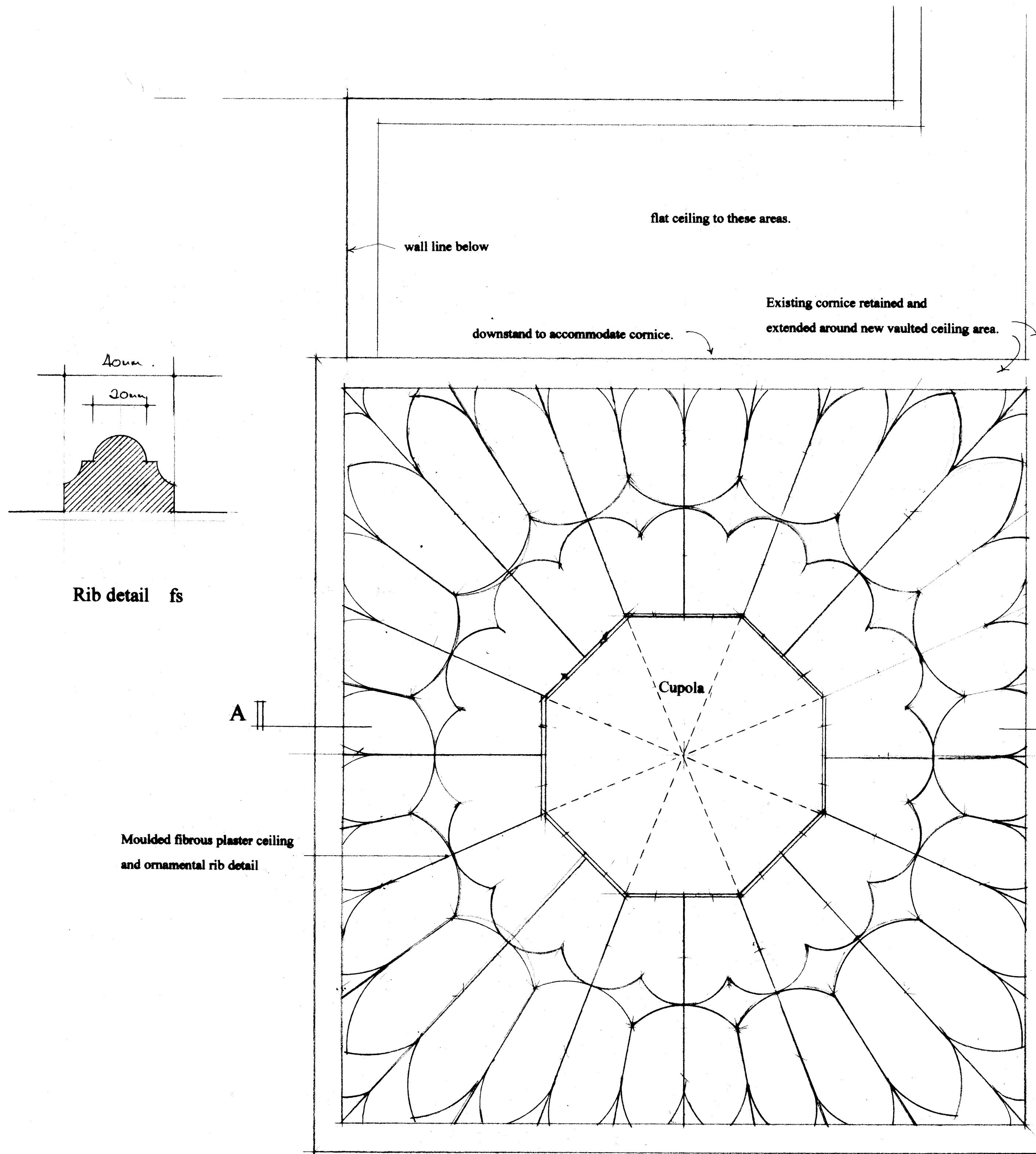
Ceiling plan 1:20
