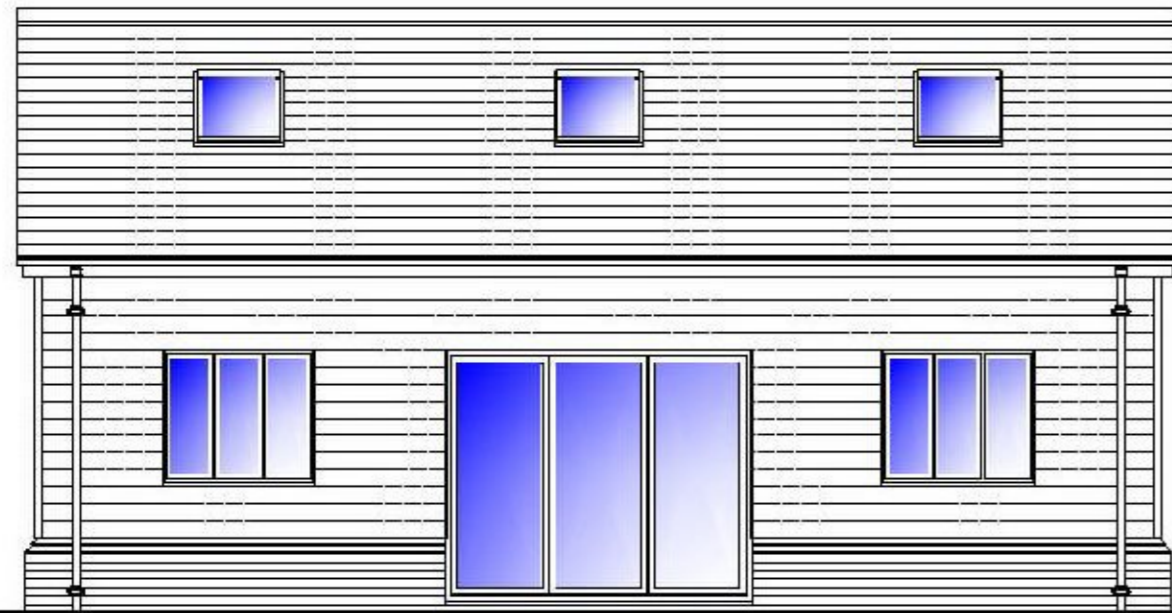
SOUTH ELEVATION
