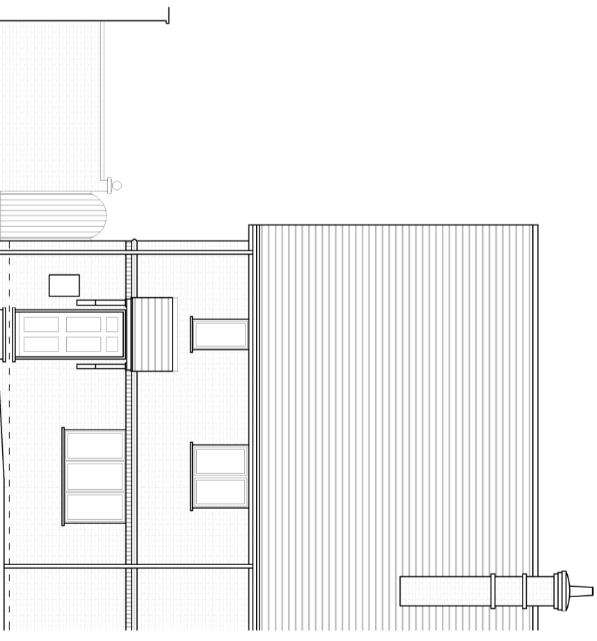
West Elevation
