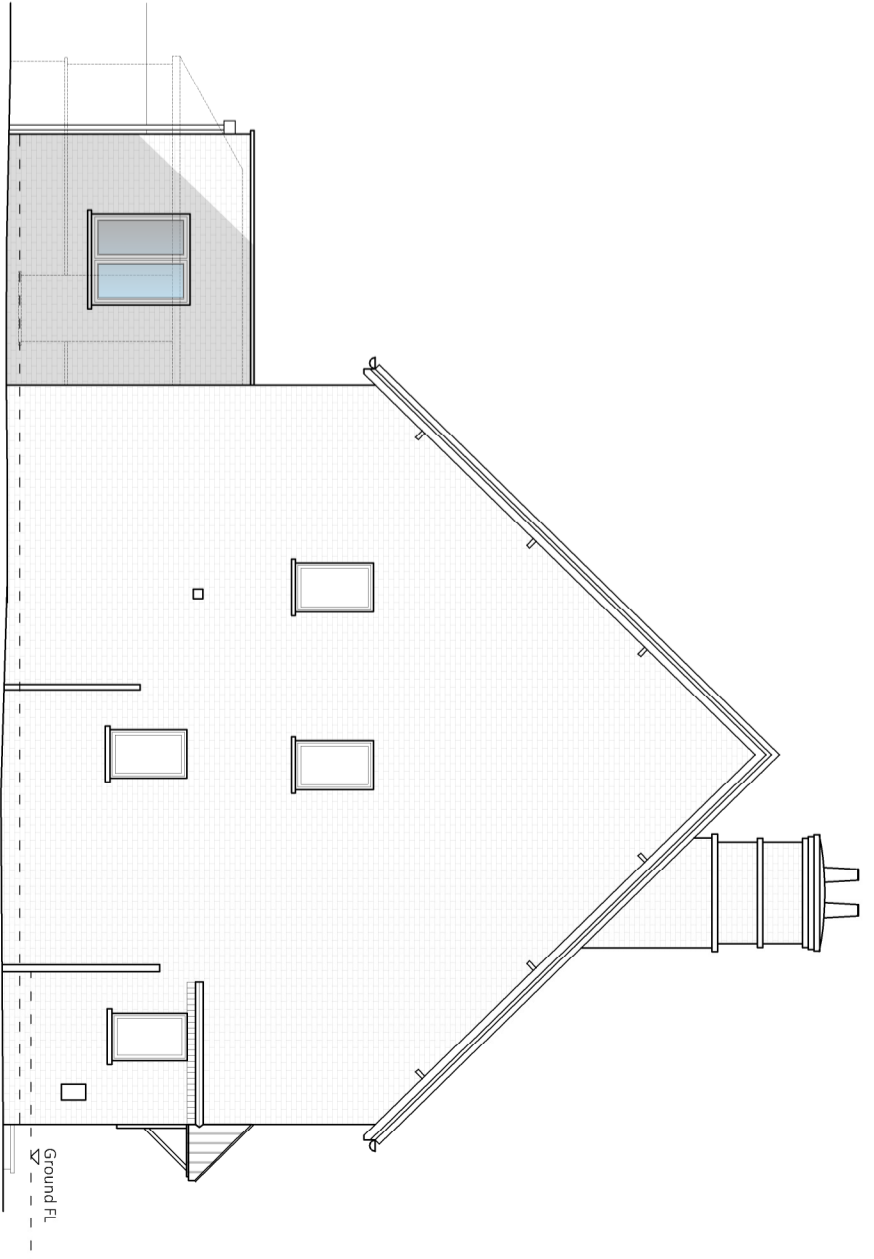
North Elevation
