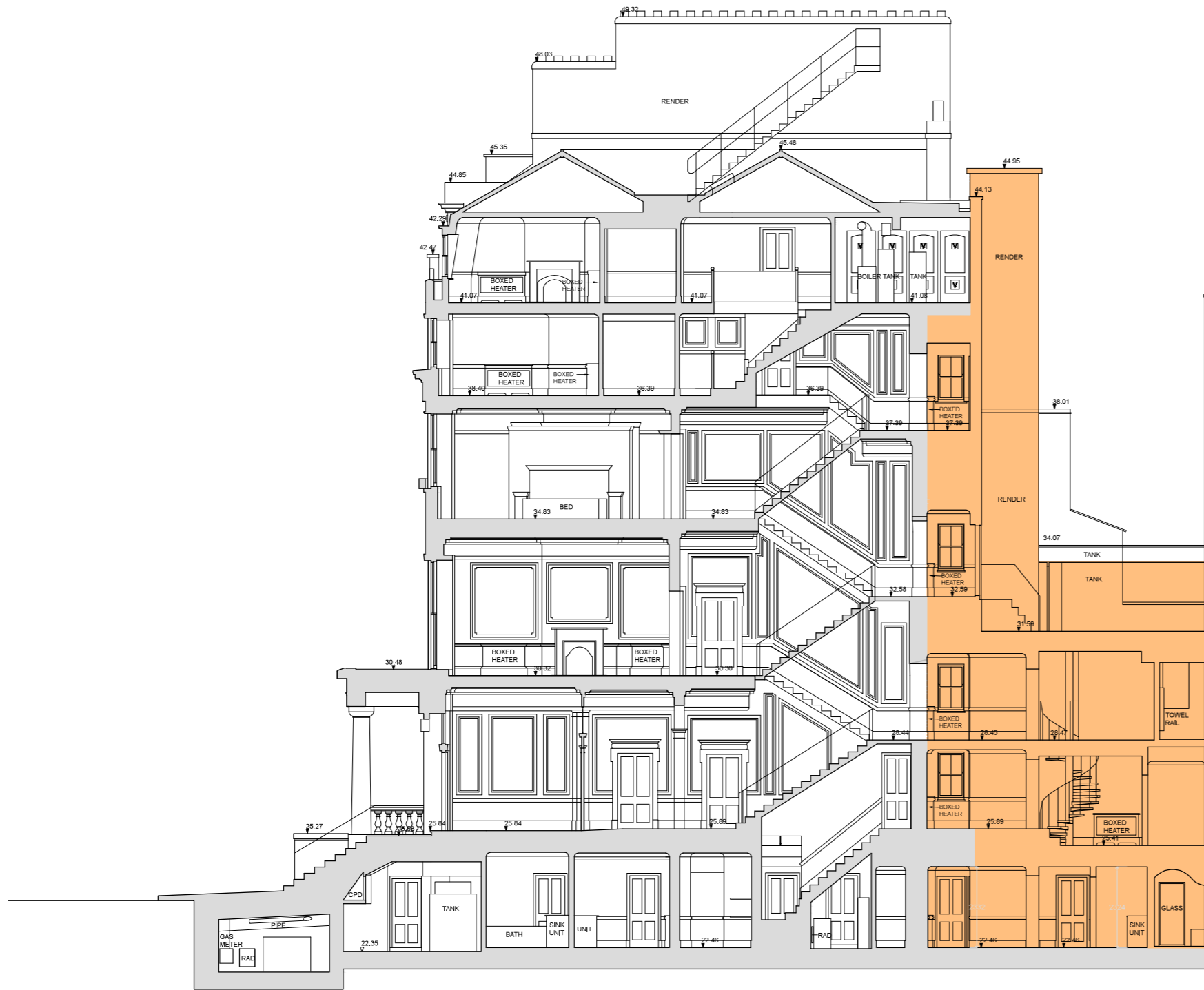
1 EXISTING SECTION B-B
