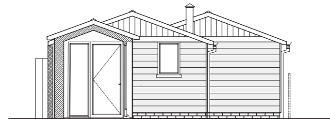
Proposed Section AA / West Elevation
