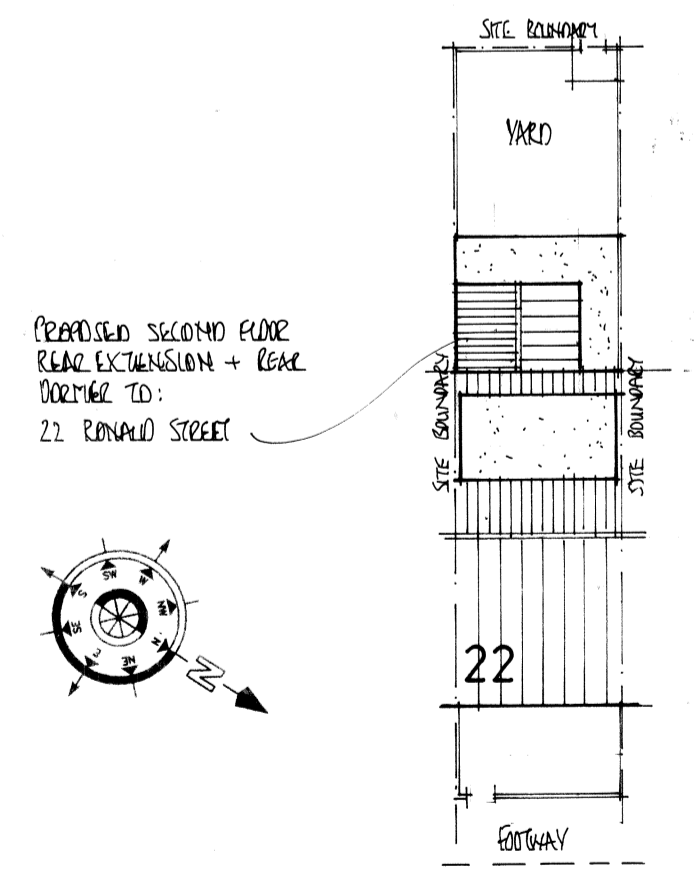
Roof & Site Plan Scale 1:200
