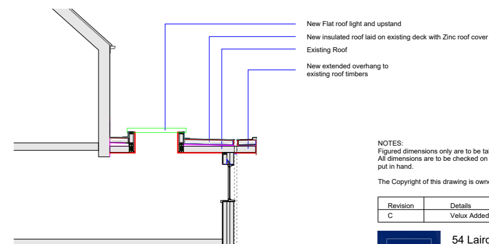
Typical section through roof light. 1:100
