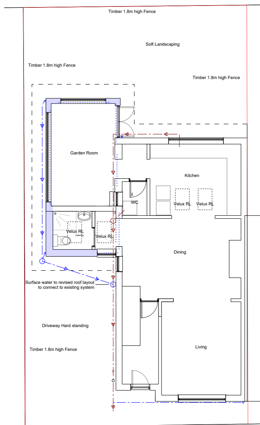
Proposed Site Plan 1:100
