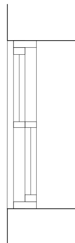
Plan and section through existing sash and case window
