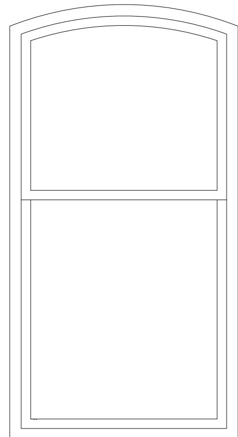
Plan and section through existing sash and case window
