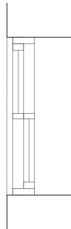
Plan and section through proposed sash and case window
