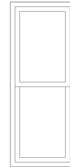
Plan and section through proposed sash and case window
