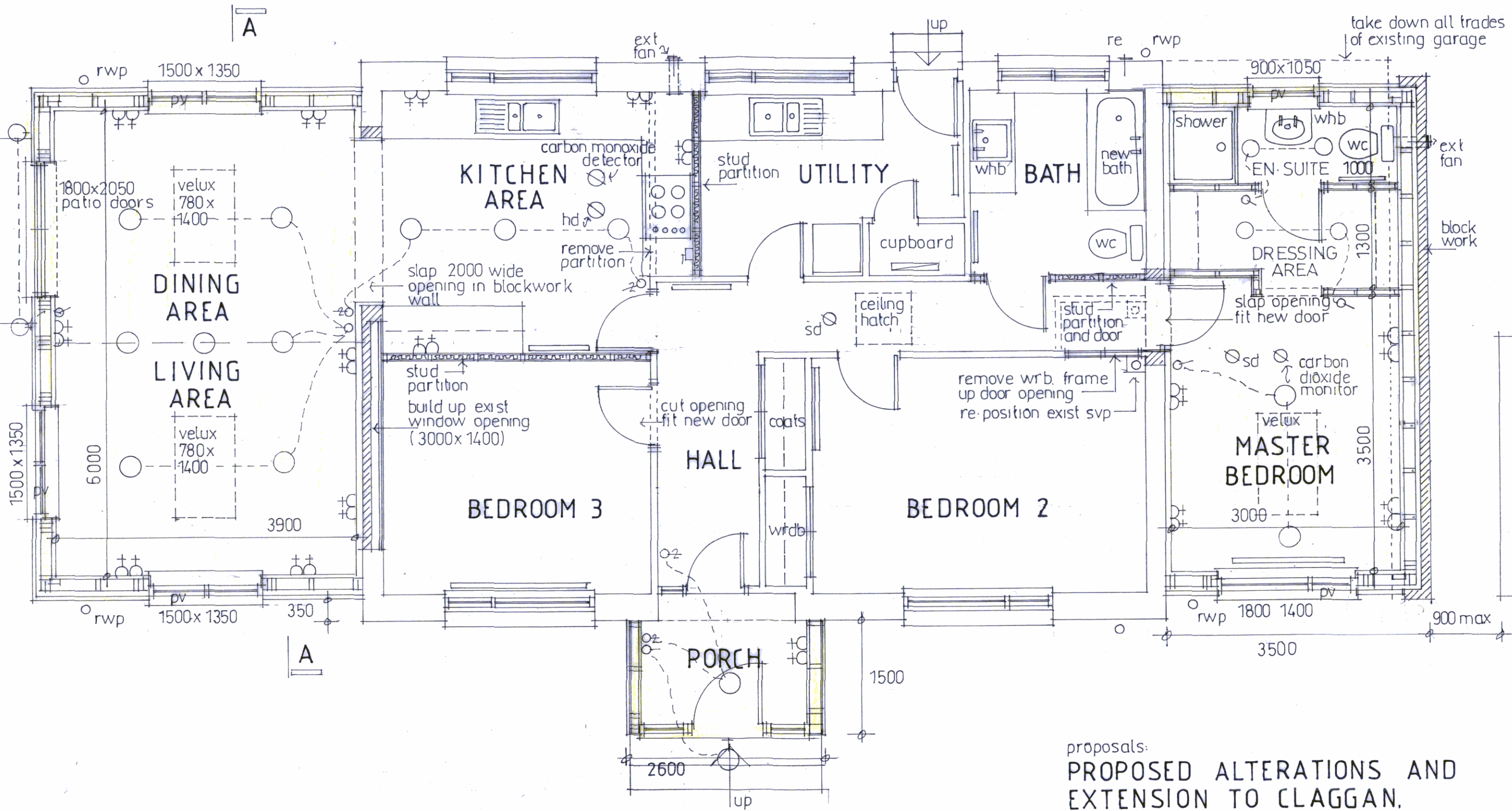
GROUND FLOOR PLAN 1 0 1 2 3 4 scale of metres! 1:50
