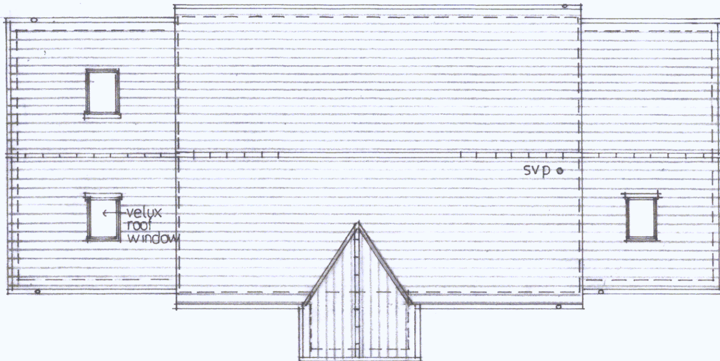
PLAN OF ROOF as proposed
