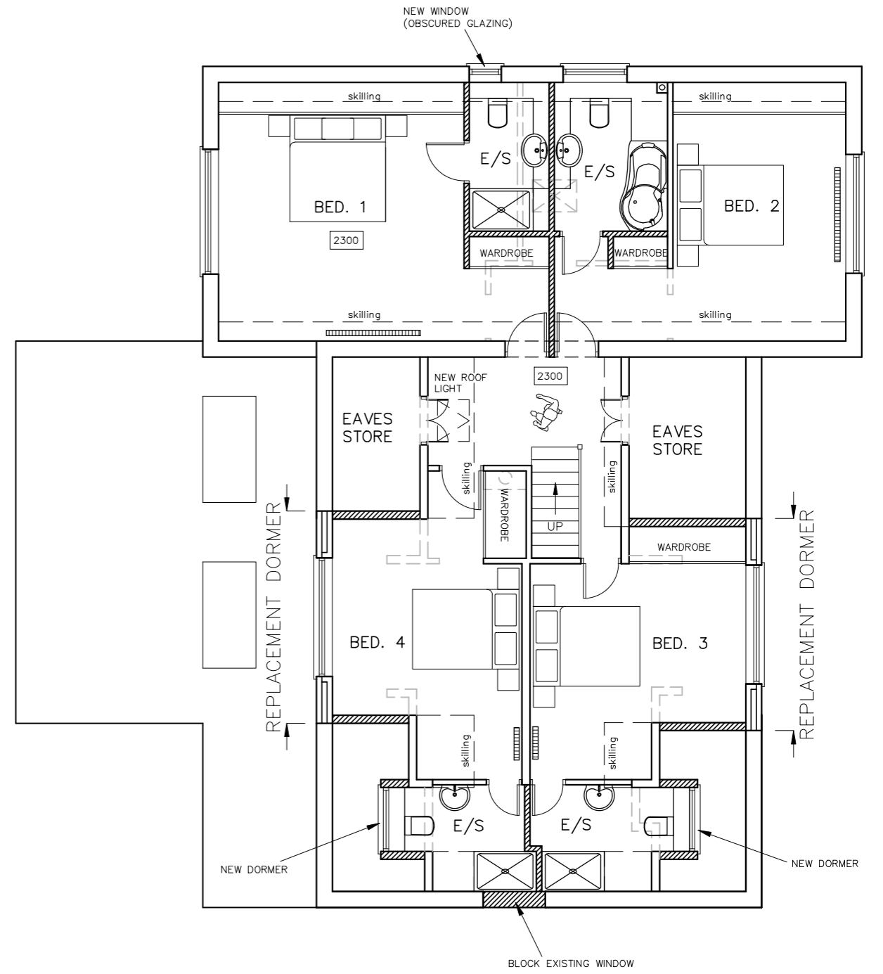
FIRST FLOOR
