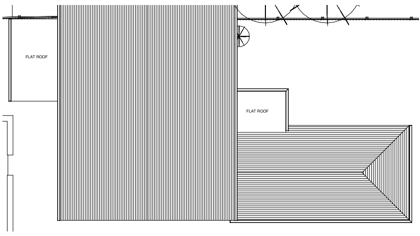
5 PROPOSED ROOF PLAN 1 : 50
