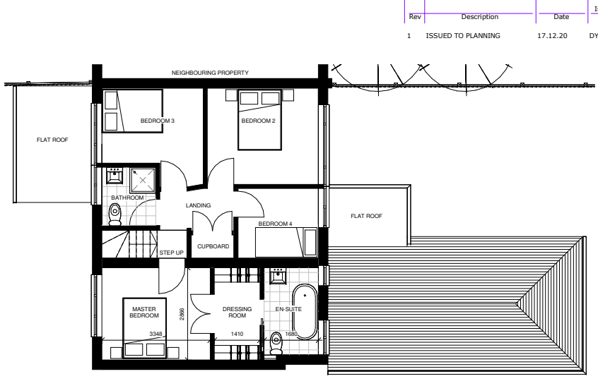
4 PROPOSED FIRST FLOOR PLAN 1 : 50
