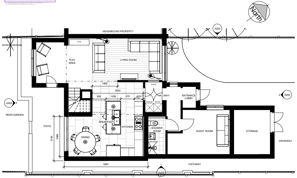
3 PROPOSED GROUND FLOOR PLAN 1 : 50
