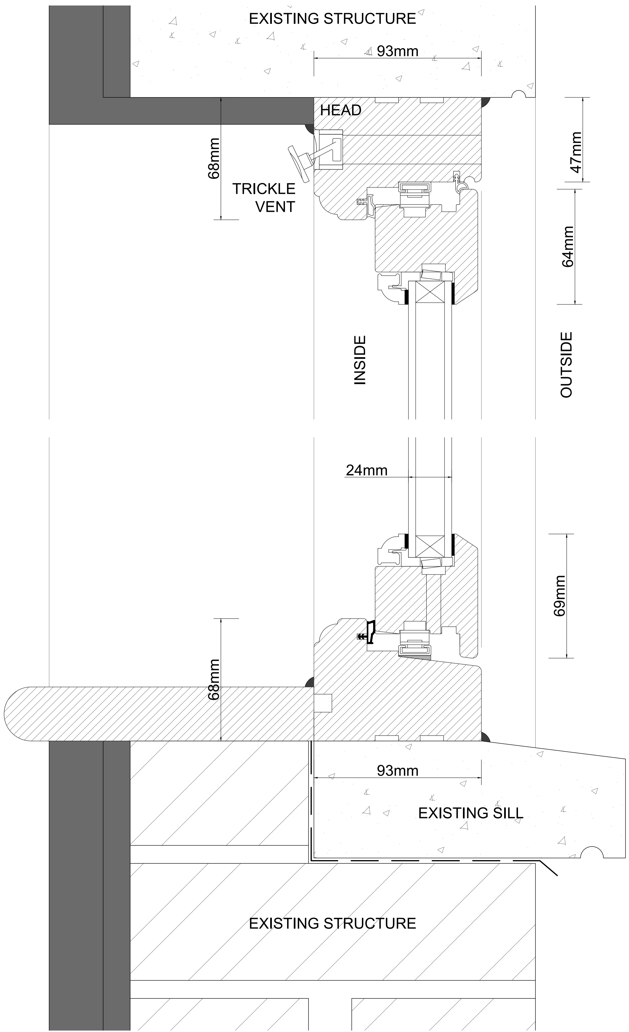
Details: Vertical Section through Proposed Timber Casement Window Scale 1:2 @ A3 | 1:1 @ A1
