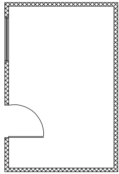
PROPOSED FLOOR PLAN OF OUTHOUSE 1:100
