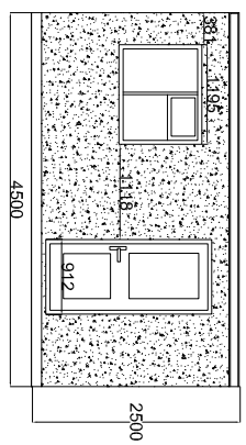
PROPOSED FRONT ELEVATION OF OUTHOUSE 1:100
