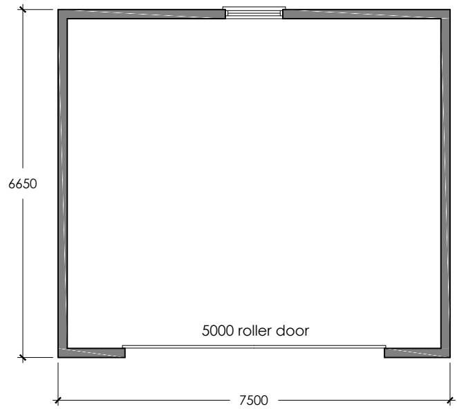
Floor Plan
