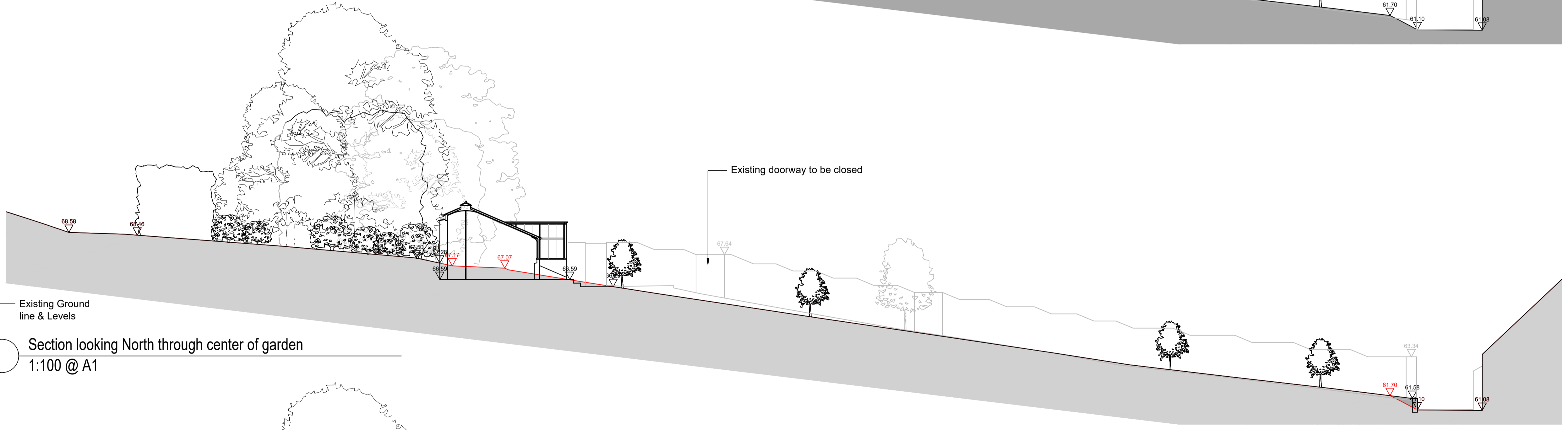
Existing section looking North through center of garden 1:100 @ A1
