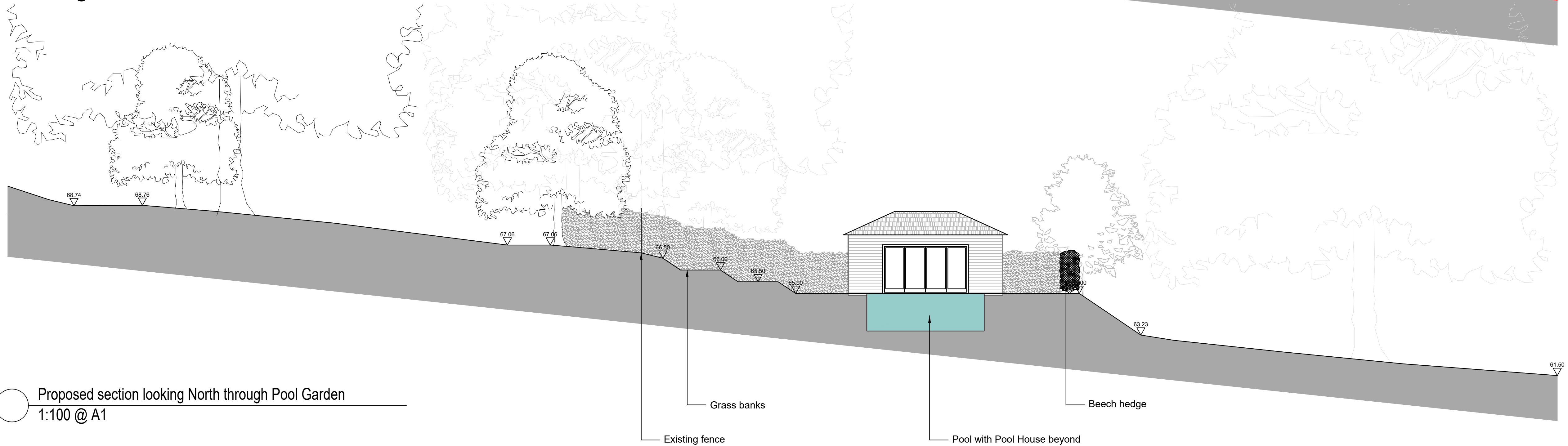
Section looking North through Pool Garden 1:100 @ A1
