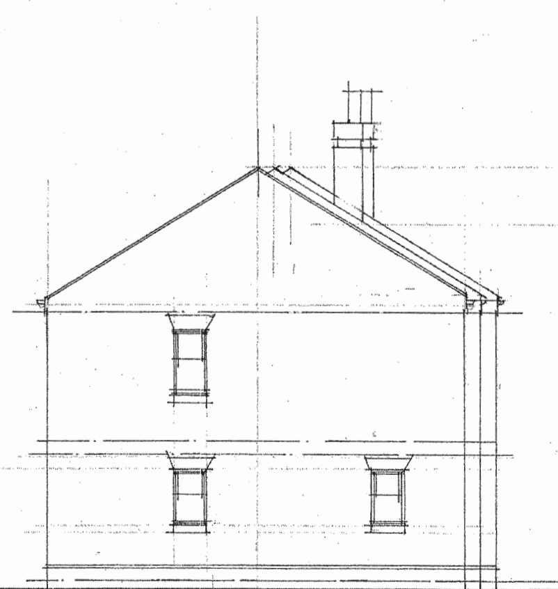
SOUTH WEST ELEVATION TO HOUSES
