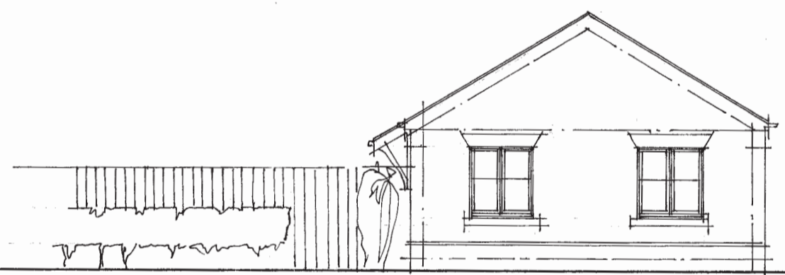
PLOT 4 SOUTH ELEVATION.
