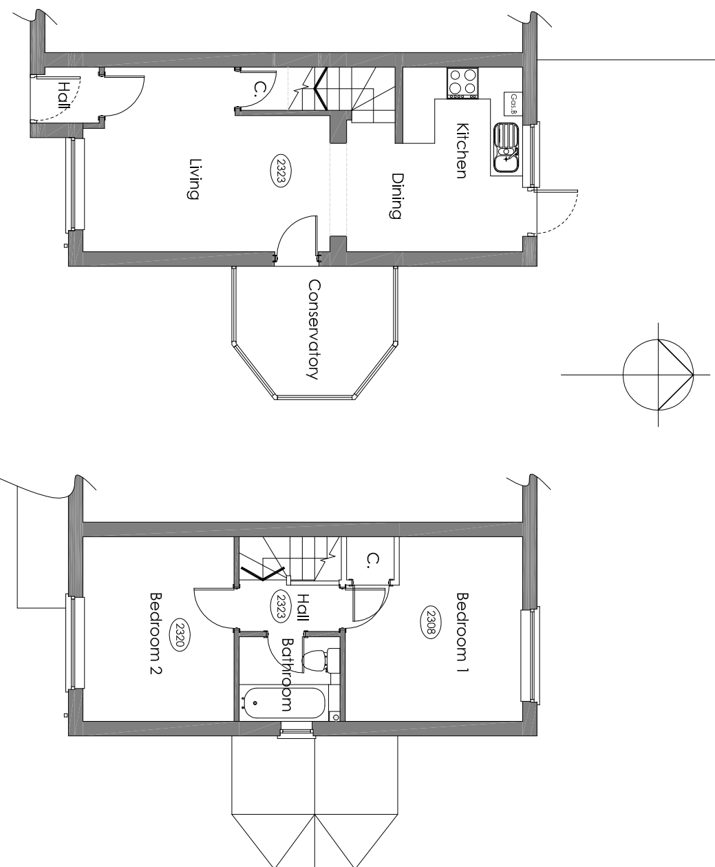
GROUND FLOOR PLAN FIRST FLOOR PLAN
