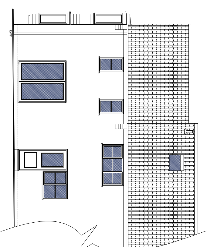
NORTH ELEVATION
