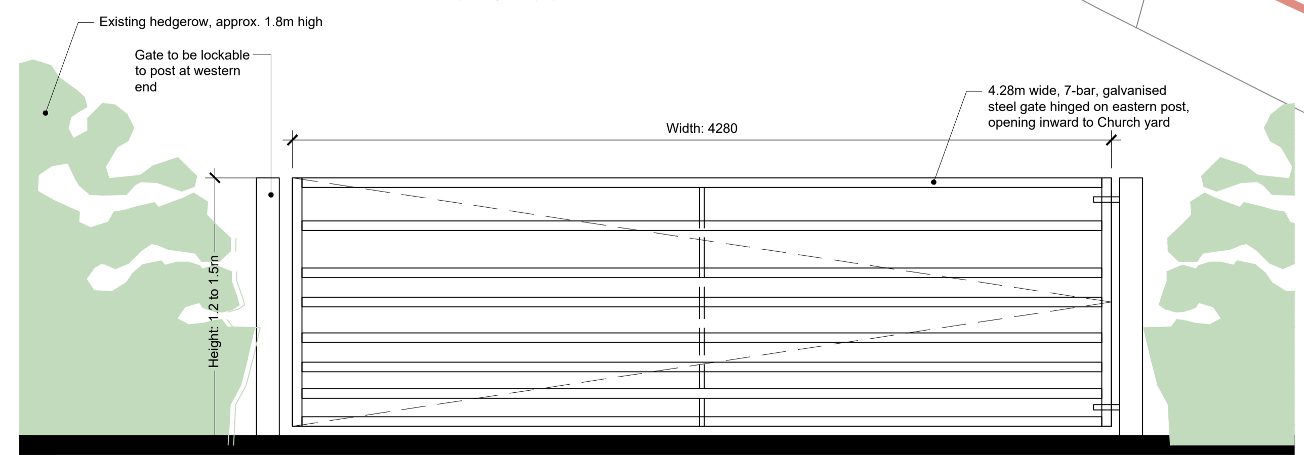
Elevation of Proposed Vehicular Access Gate 1:20
