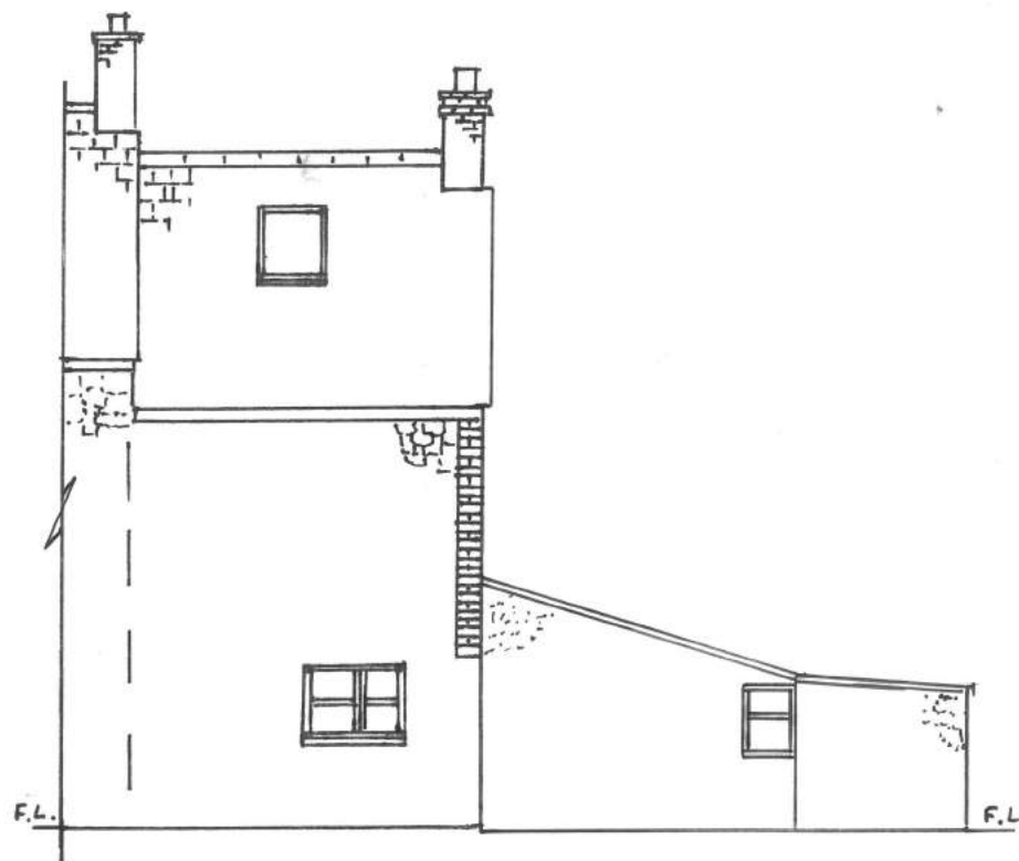
West Elevation
