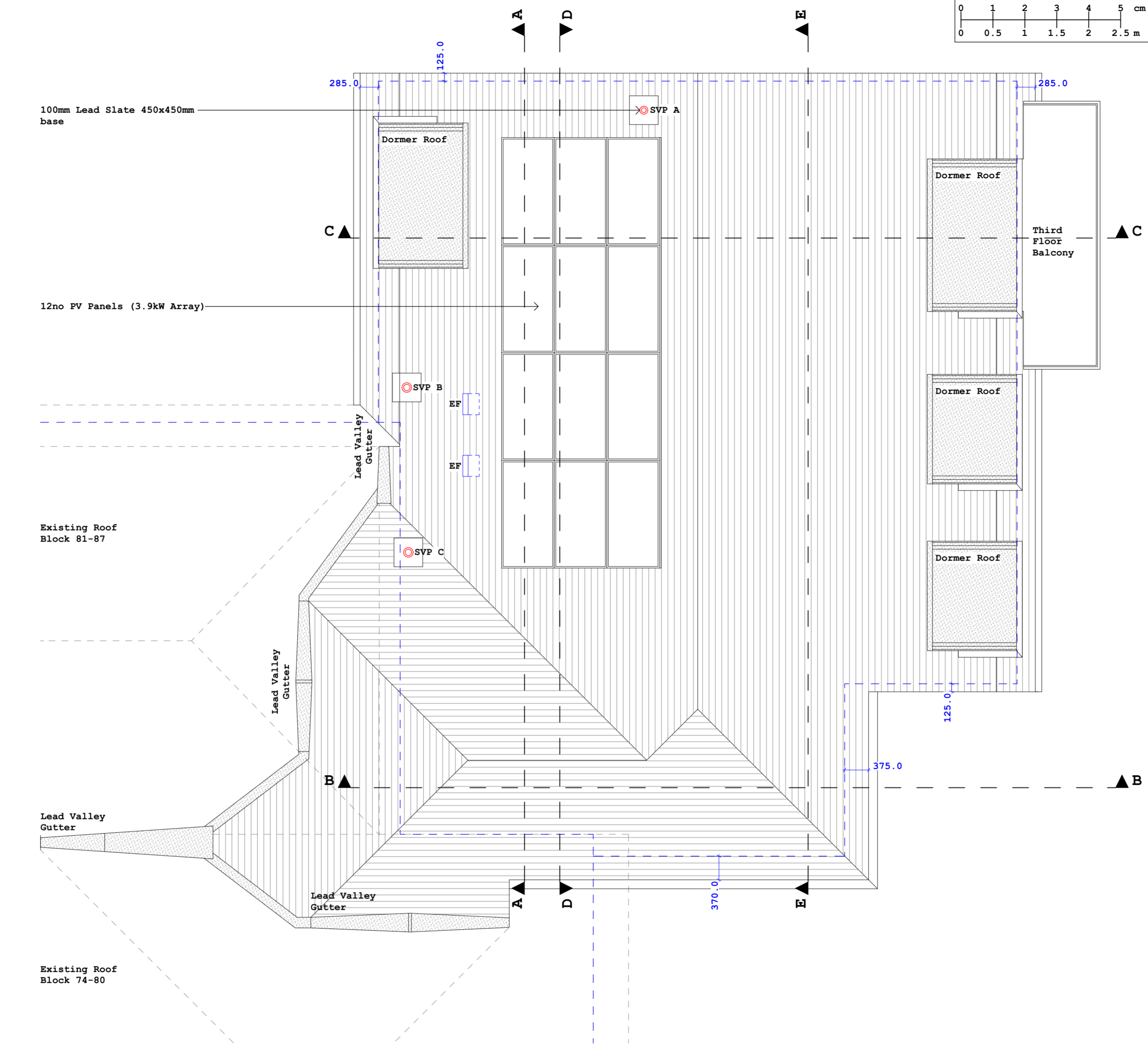
ROOF GENERAL ARRANGEMENT PLAN
