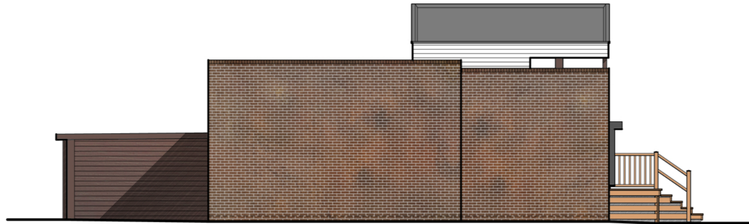
South-West Elevation
