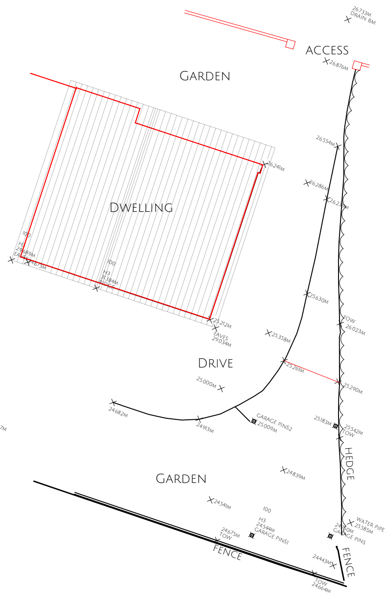
SITE PLAN 0 2M 4M 6M 8M 10M 1:200
