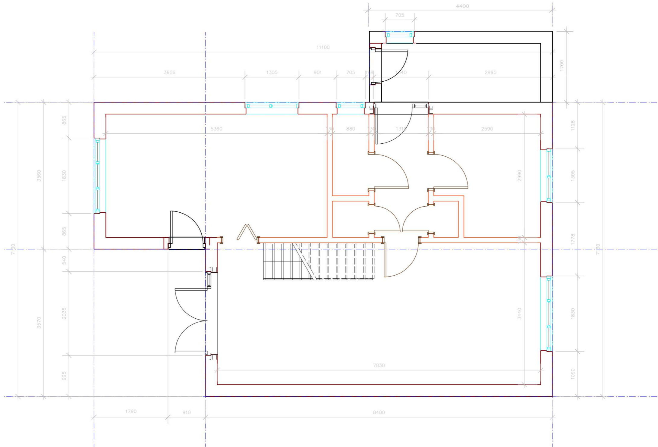
01 Ground Floor Plan 1:50
