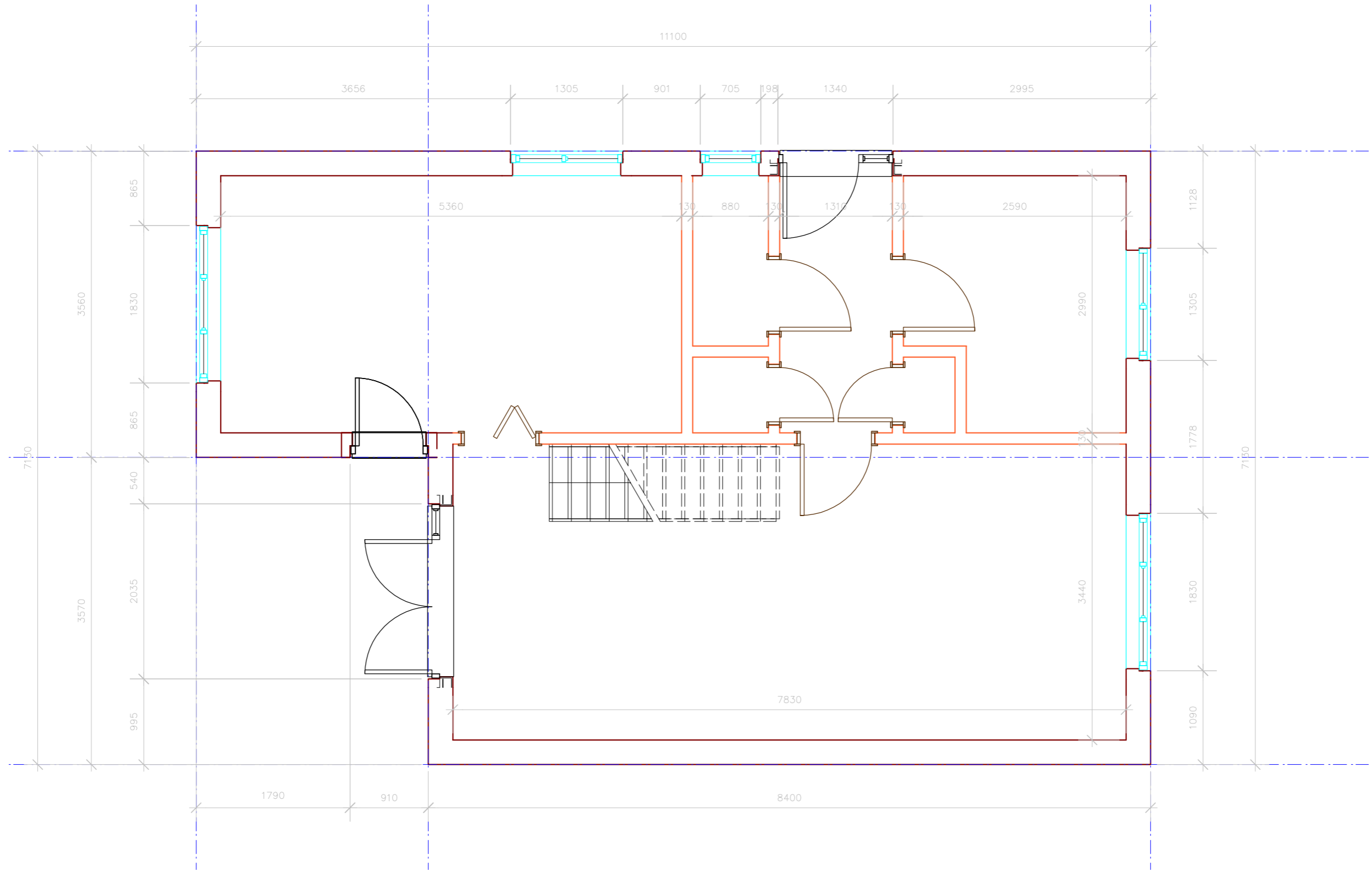
01 Ground Floor Plan 1:50
