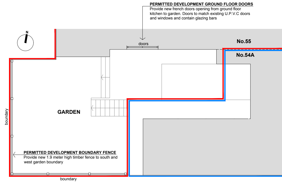
PROPOSED GARDEN BLOCK PLAN
