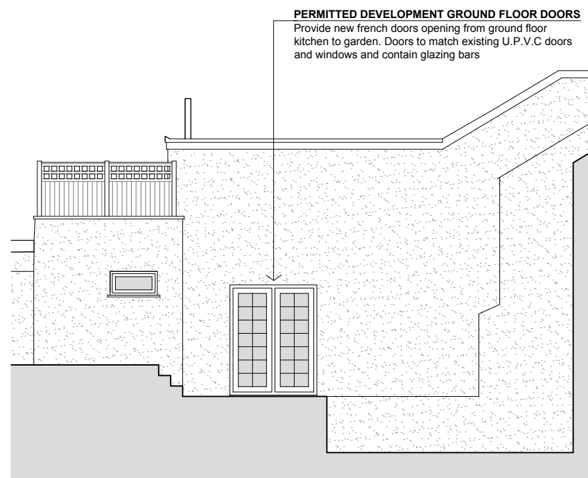
PROPOSED REAR ELEVATION (SOUTH)
