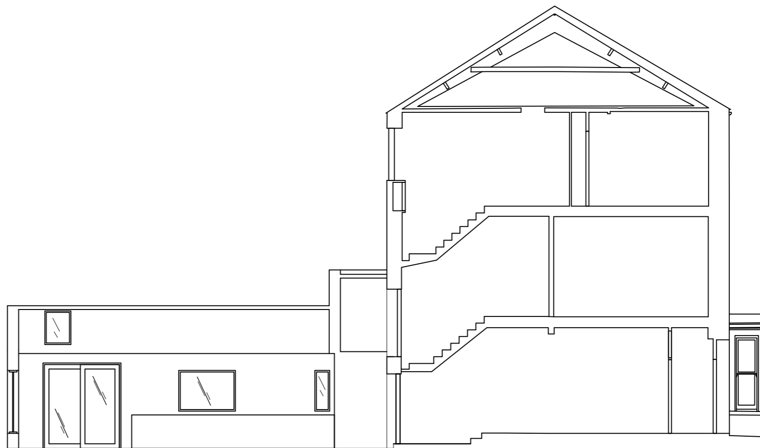
Proposed South Section
