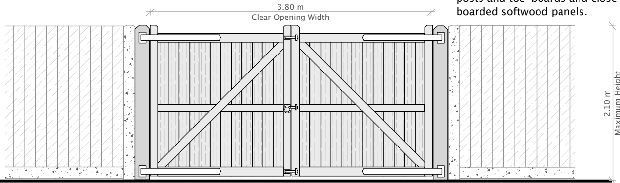
GATE ELEVATION 1:50 (From Garden / Driveway)
