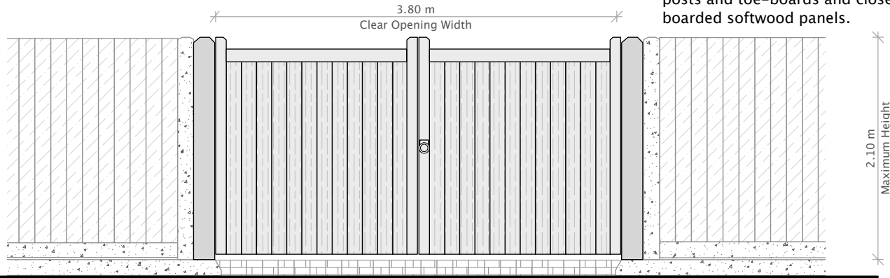
GATE ELEVATION 1:50 (From Car Park)
