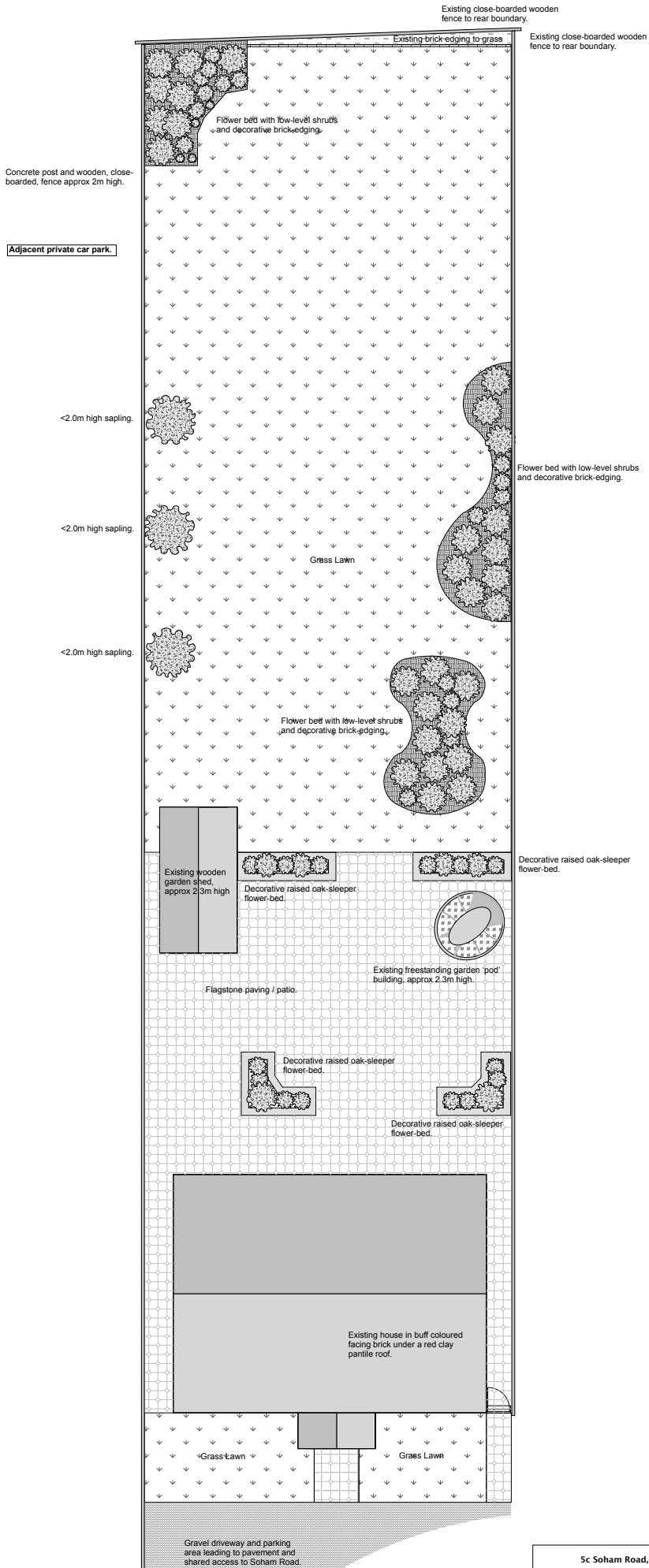
Existing Site Plan 1:200
