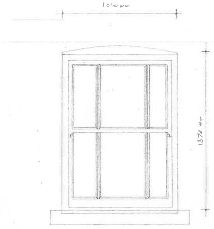
WINDOW ELEVATION 1-20
