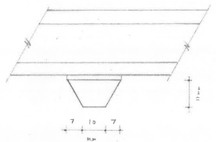
BONDED GLAZING BEAD 1-1
