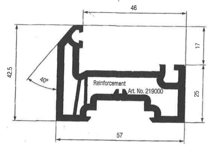
mid sash
