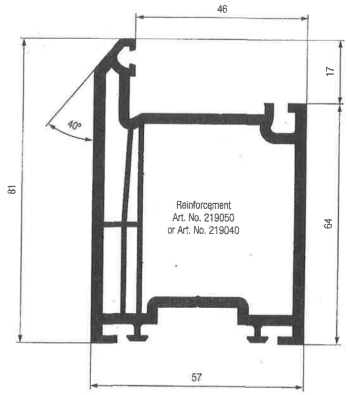
bottom sash
