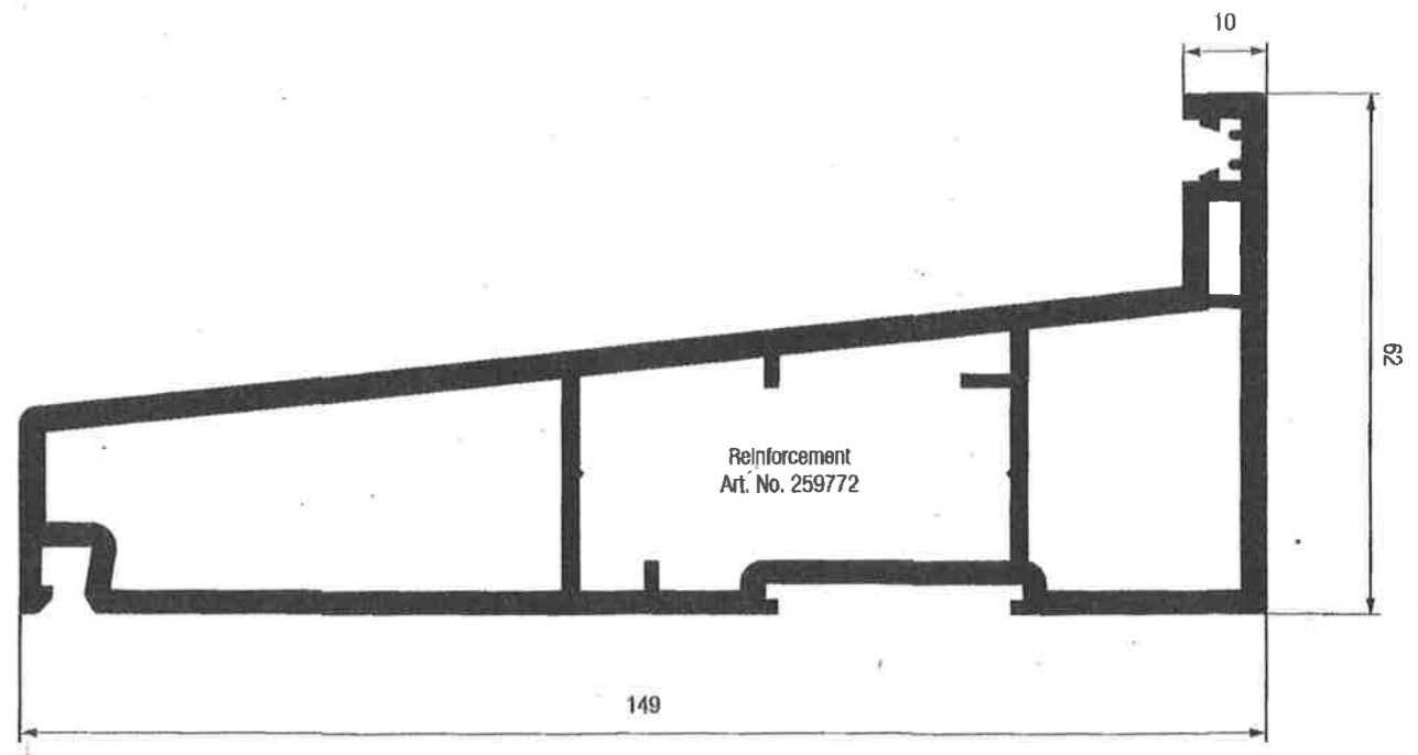
sill
