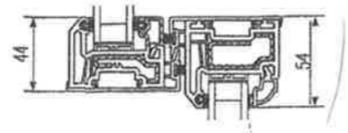
mid sash
