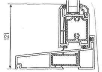
sill
