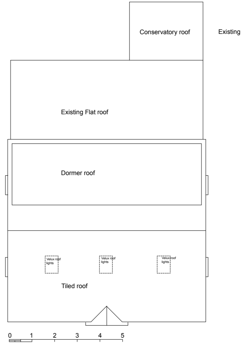
Proposed roof plan 1:100 Scale
