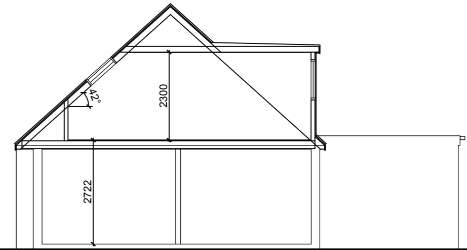
Proposed Section
