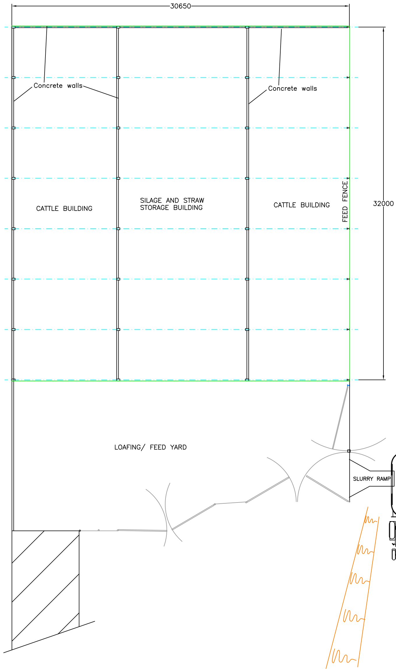
EXISTING PLAN VIEW OF FARM YARD
