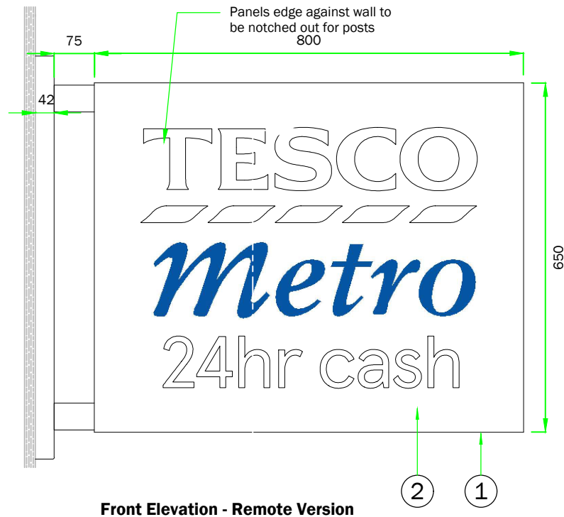
Front Elevation - Remote Version scale 1:10
