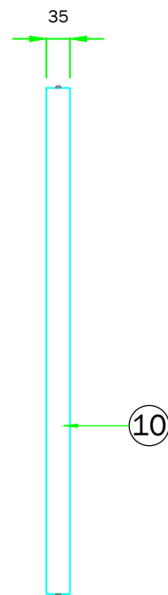
Shroud: End Elevation scale 1:10
