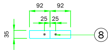
Shroud: Plan View scale 1:10
