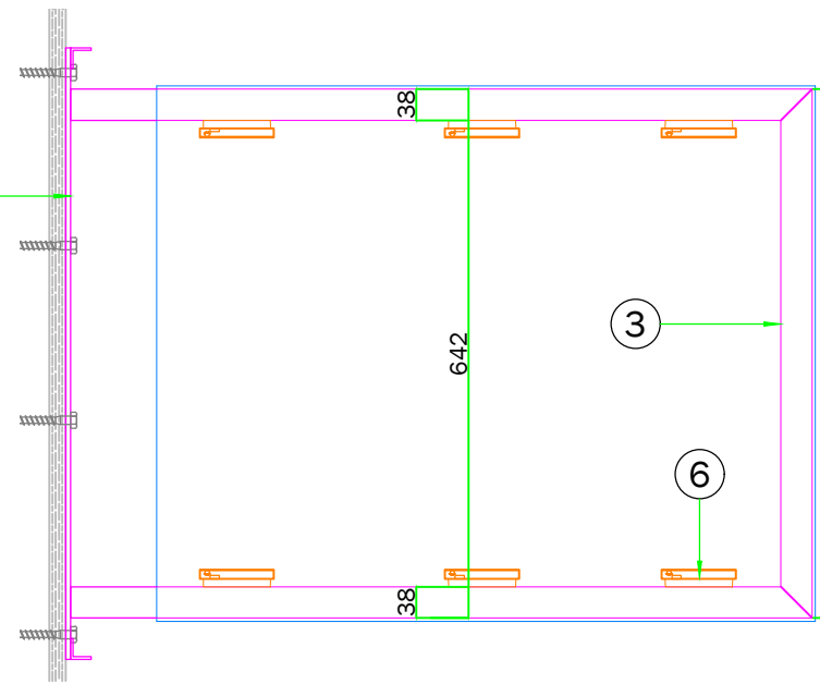
Framework: Front Elevation scale 1:10
