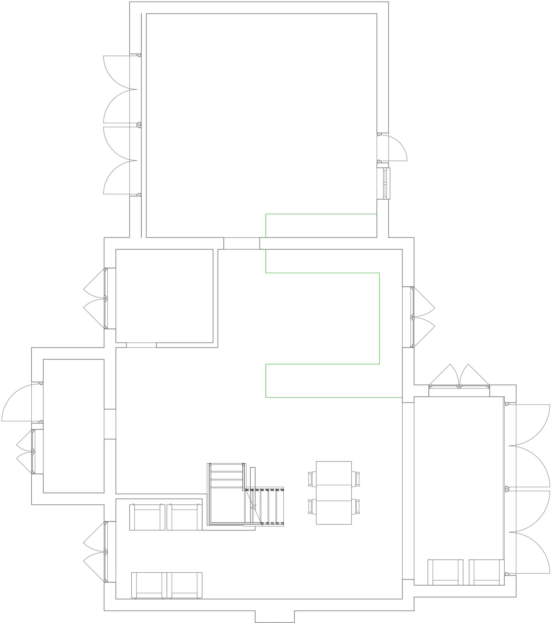
1 Ground Existing 1 : 50
