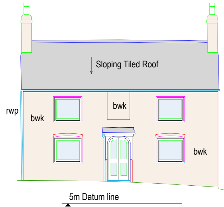
East Elevation
