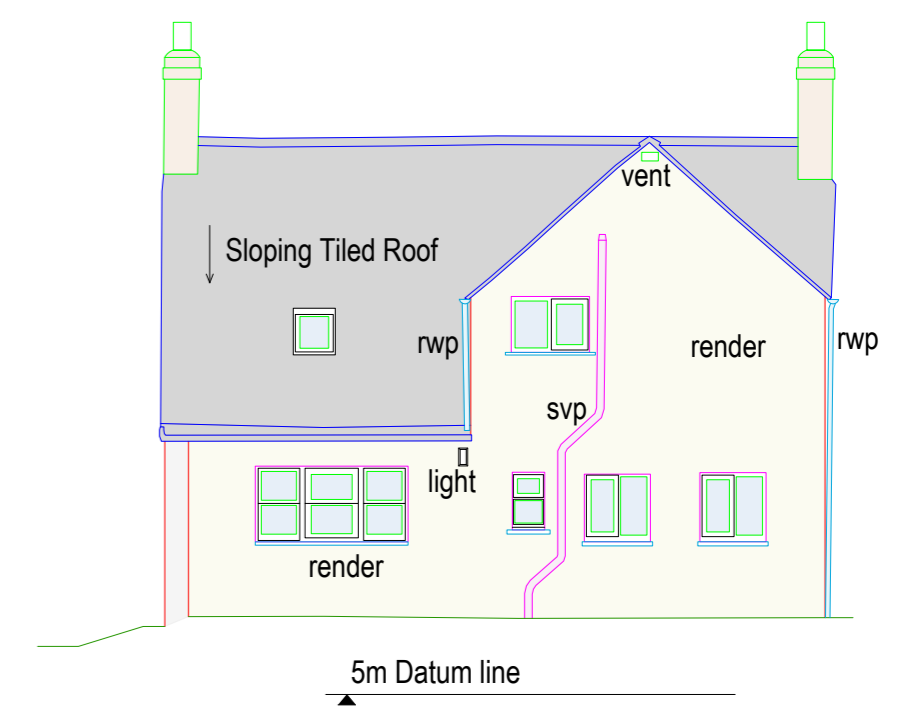
West Elevation
