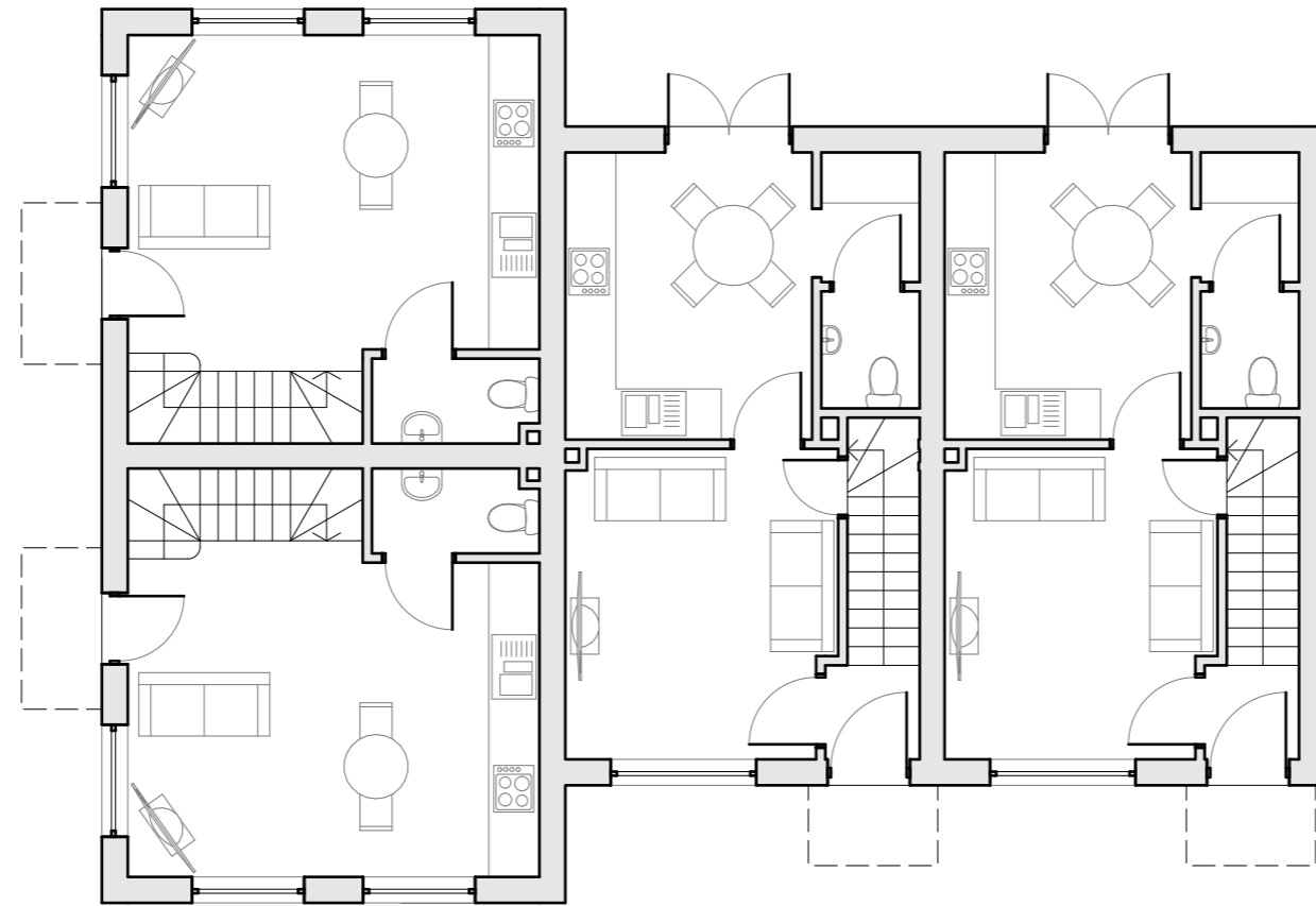
House Types 'A' & 'N' Ground Floor Plan (Units 1 to 8) 1:100
