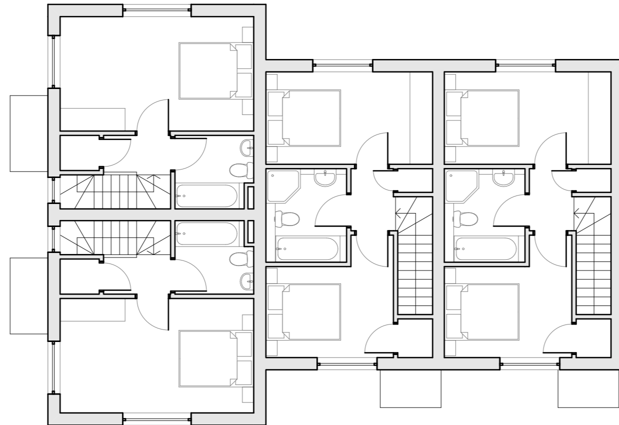
House Types 'A' & 'N' First Floor Plan (Units 1 to 8) 1:100
