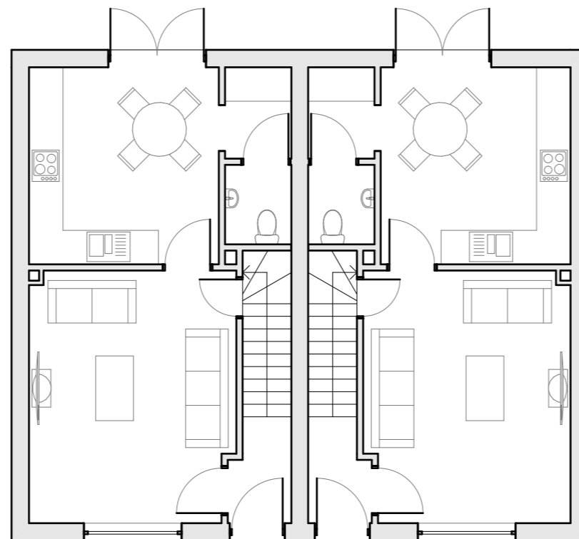
House Types 'R' Ground Floor Plan (Units 13-14, 26-27) 1:100
