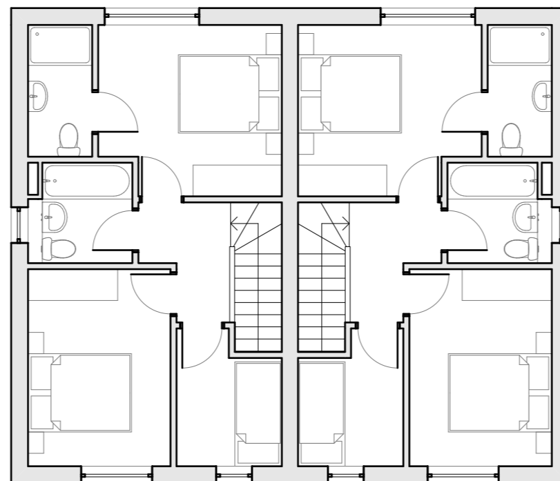
House Types 'R' First Floor Plan (Units 13-14, 26-27) 1:100
