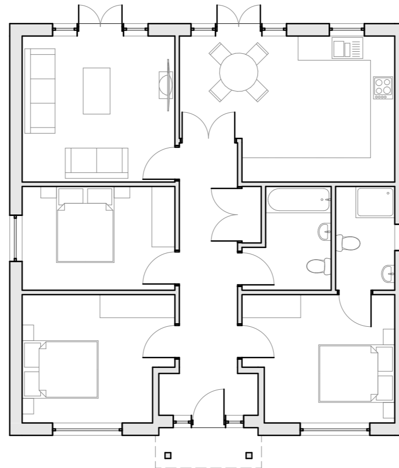
House Type 'L' Ground Floor Plan (Units 22 & 23) 1:100
