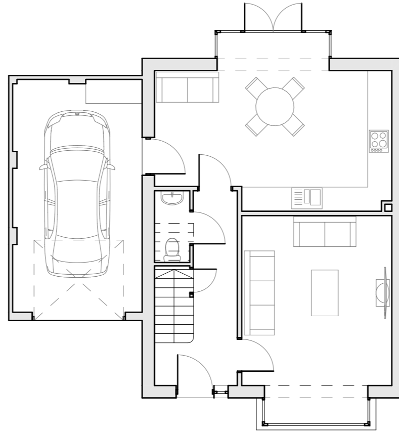
House Type 'O' Ground Floor Plan (Units 24, 25 & 28) 1:100
