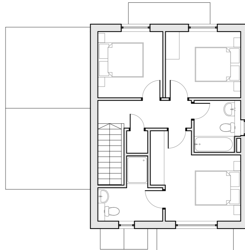
House Type 'O' First Floor Plan (Units 24, 25 & 28) 1:100
