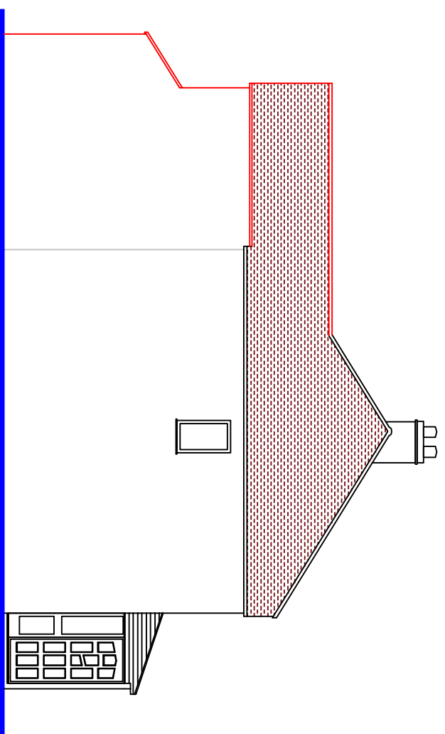
LEFT SIDE ELEVATION (Proposed)
