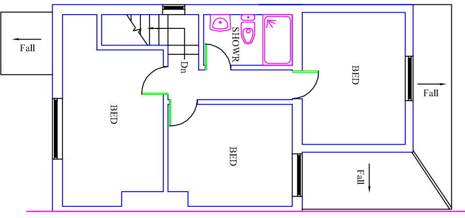
FIRST FLOOR PLAN PROPOSED
