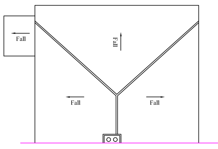
ROOF PLAN
