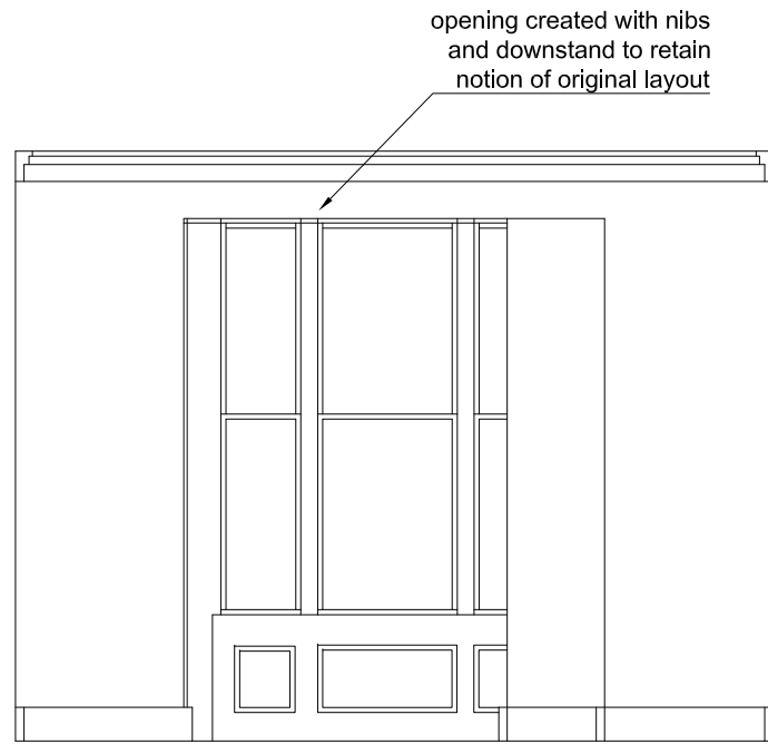
01 Elevation O Scale 1:50
