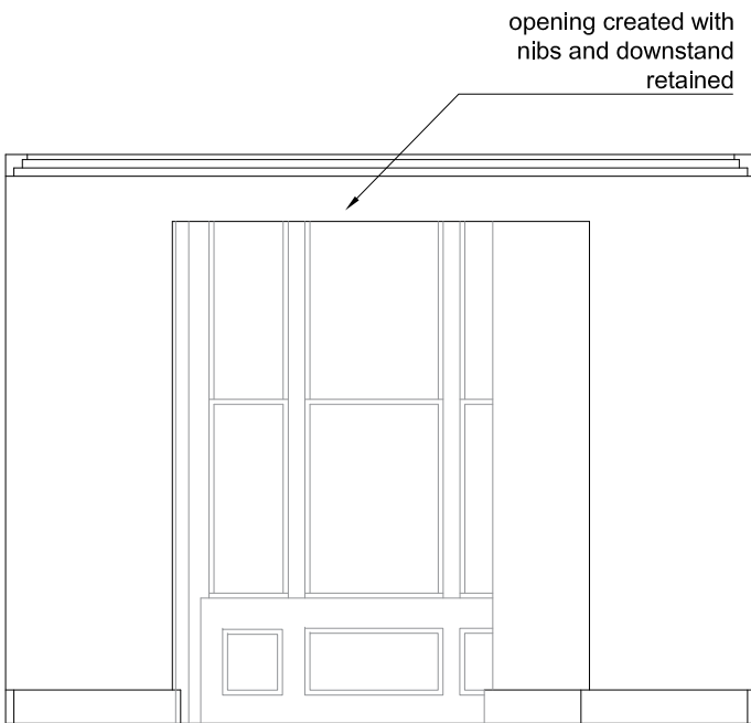
01 Elevation R Scale 1:50
