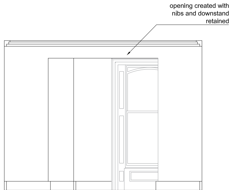
02 Elevation S Scale 1:50
