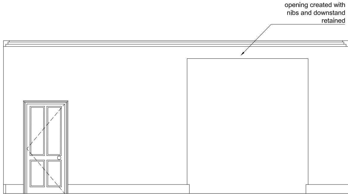
03 Elevation Q Scale 1:50
